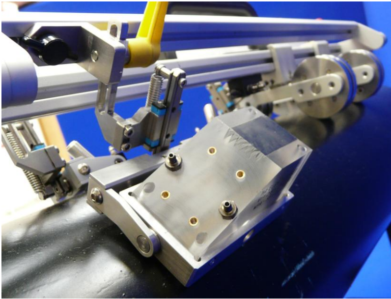
Close-up of Phased Array toolpost and cradle with wedge
