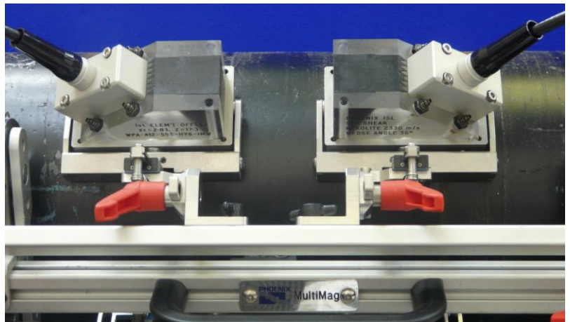
Close-up of MultiMag with 2 Phased Array probes on 6" OD pipe
